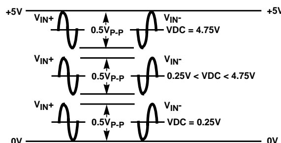
FIGURE 4. DIFFERENTIAL ANALOG INPUT COMMON MODE VOLTAGE RANGE
